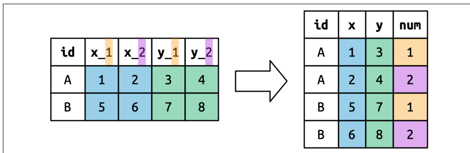
Figure 5-7. Pivoting with names_to = c(".value", "num") splits the column names into two components: the first part determines the output column name ( x or y ), and the second part determines the value of the num column.
